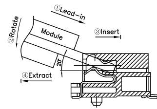
How to mate and unmate Mate: ①- ②- ③ Unmate: ④
